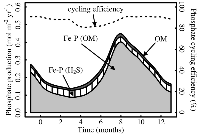
Fig. 7. Seasonal variation in phosphate production by diagenetic reactions: remineralization of organic matter (OM); dissolution of iron oxyhydroxides during dissimilatory iron reduction ( \text{Fe-P (OM)} ); and dissolution of iron oxyhydroxides during iron reduction by hydrogen sulphide ( \text{Fe-P (H}_2\text{S)} ). The dotted line represents cycling efficiency, which is defined as the percentage of phosphate produced at a time that is taken up by iron oxyhydroxide formation.
